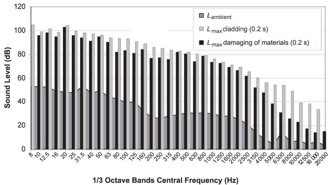
Figure 4. Spectrum of the level of exposure to sound pressure (in Trzebień), explosion No. 2.
